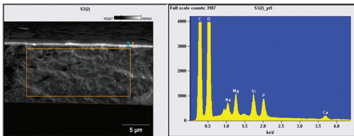
Figure 5. Low-magnification SEM image and corresponding EDX spectrum for the cross-section of a 95:5 rye arabinoxylan (RAX)-sepiolite composite film.
